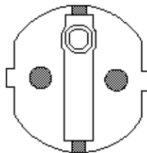
PECO Plug #141-1-075 10-16 Amps 250 Volts CEE 7-VII
