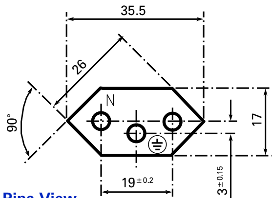
Pins View
